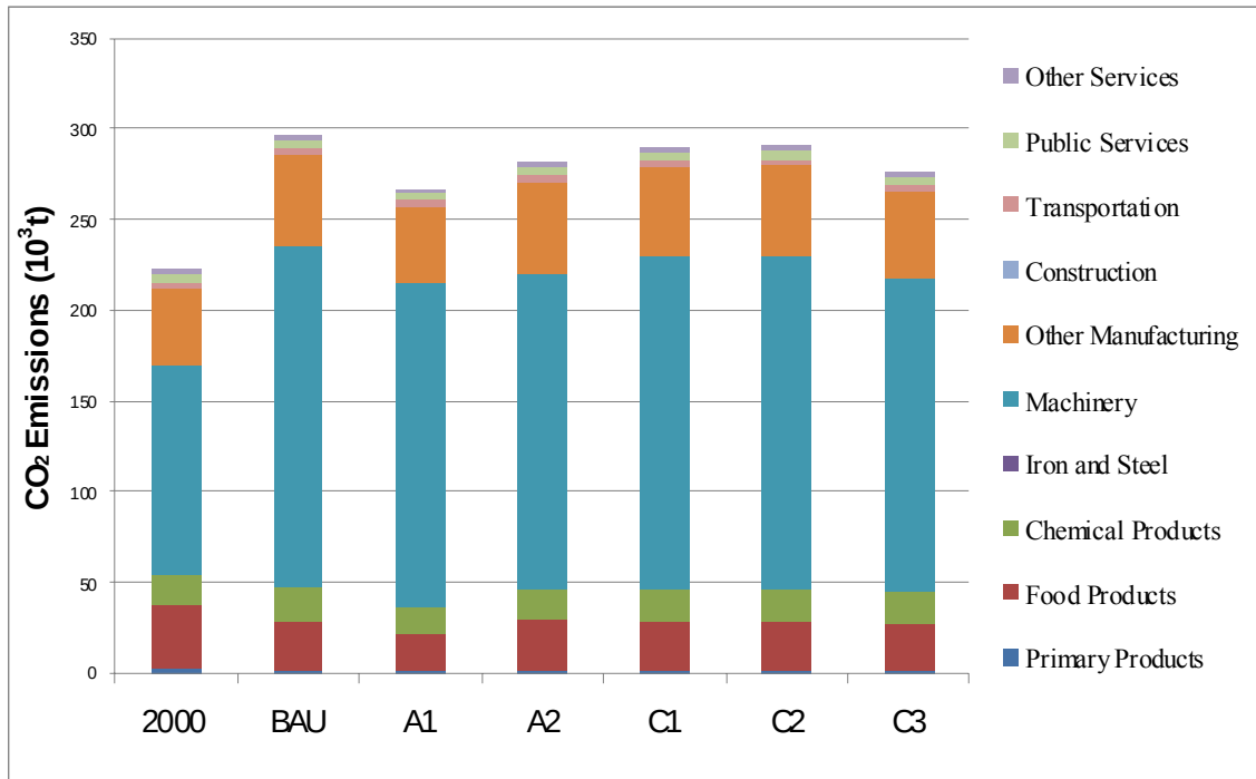
Figure 4 Sectoral amount of CO 2 Emissions in Ibaraki Driven by ROJ
