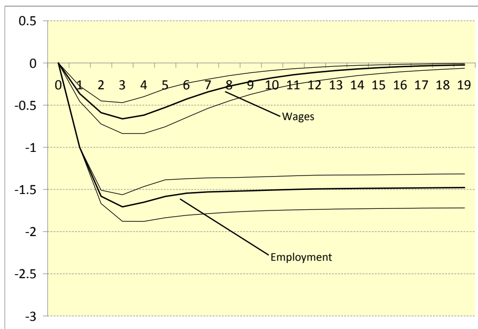
Figure 7: Impulse responses from a -1\% shock to \Delta \ln e , CTE model with 2 lags – specification with wages. Confidence bands represent a 95% confidence interval.
