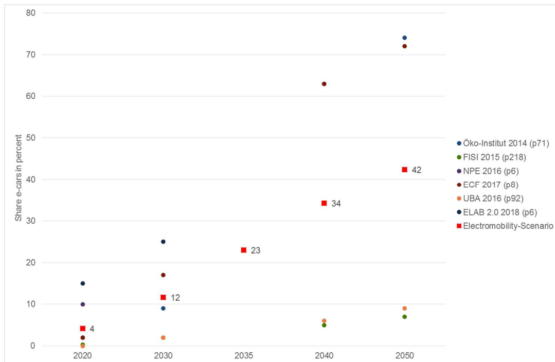
Figure 7: Market penetration of electric cars in different reference scenarios
