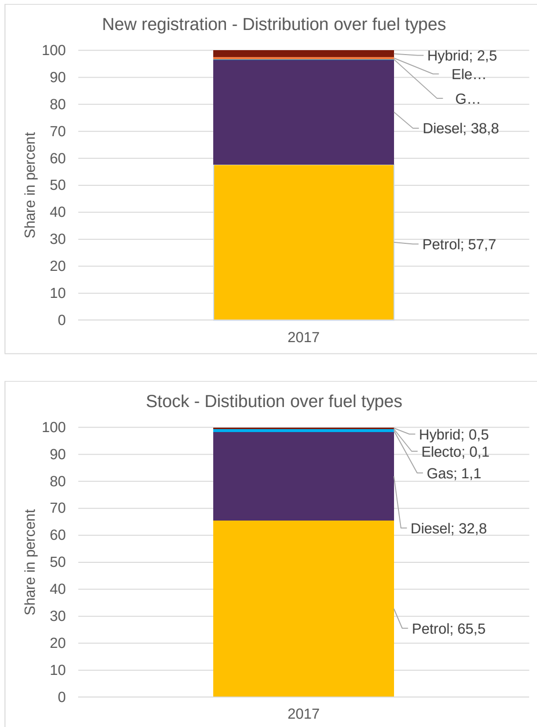
Figure 1: New passenger car registrations and passenger car stock by fuel type in 2017
