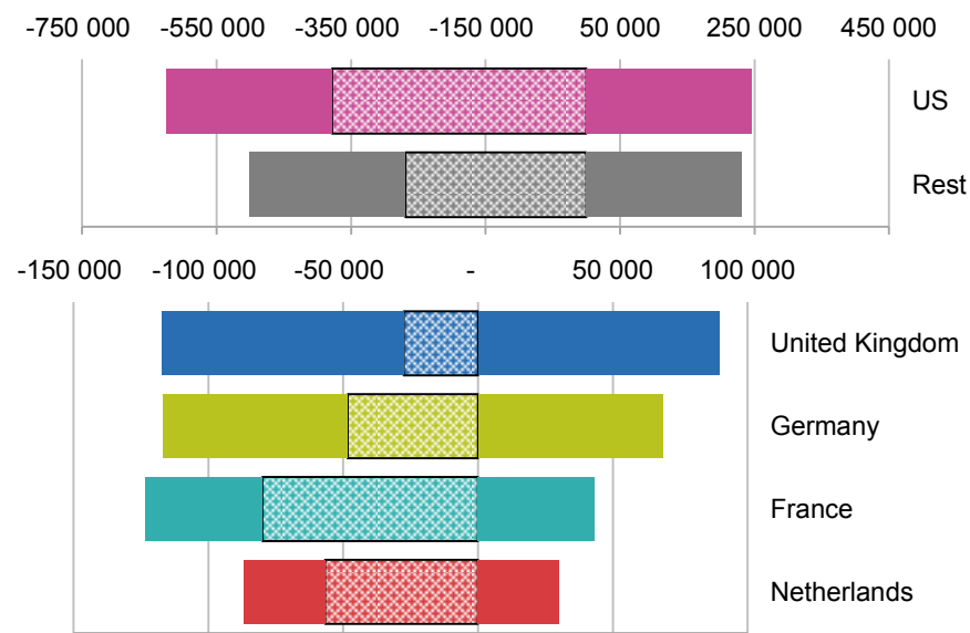
Figure 13.9: Analysis of the total column discrepancies; net and absolute discrepancies by country and by CPA products (relates to A5 in Figure 13.4)
