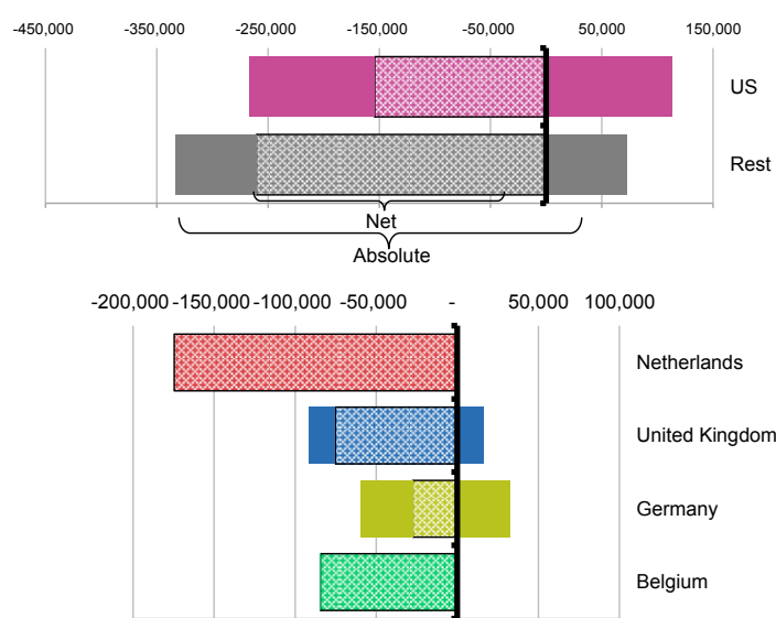
Figure 13.5: Analysis of the total row discrepancies; net and absolute sum of discrepancies by country and industries (relates to A1 in Figure 13.4).
